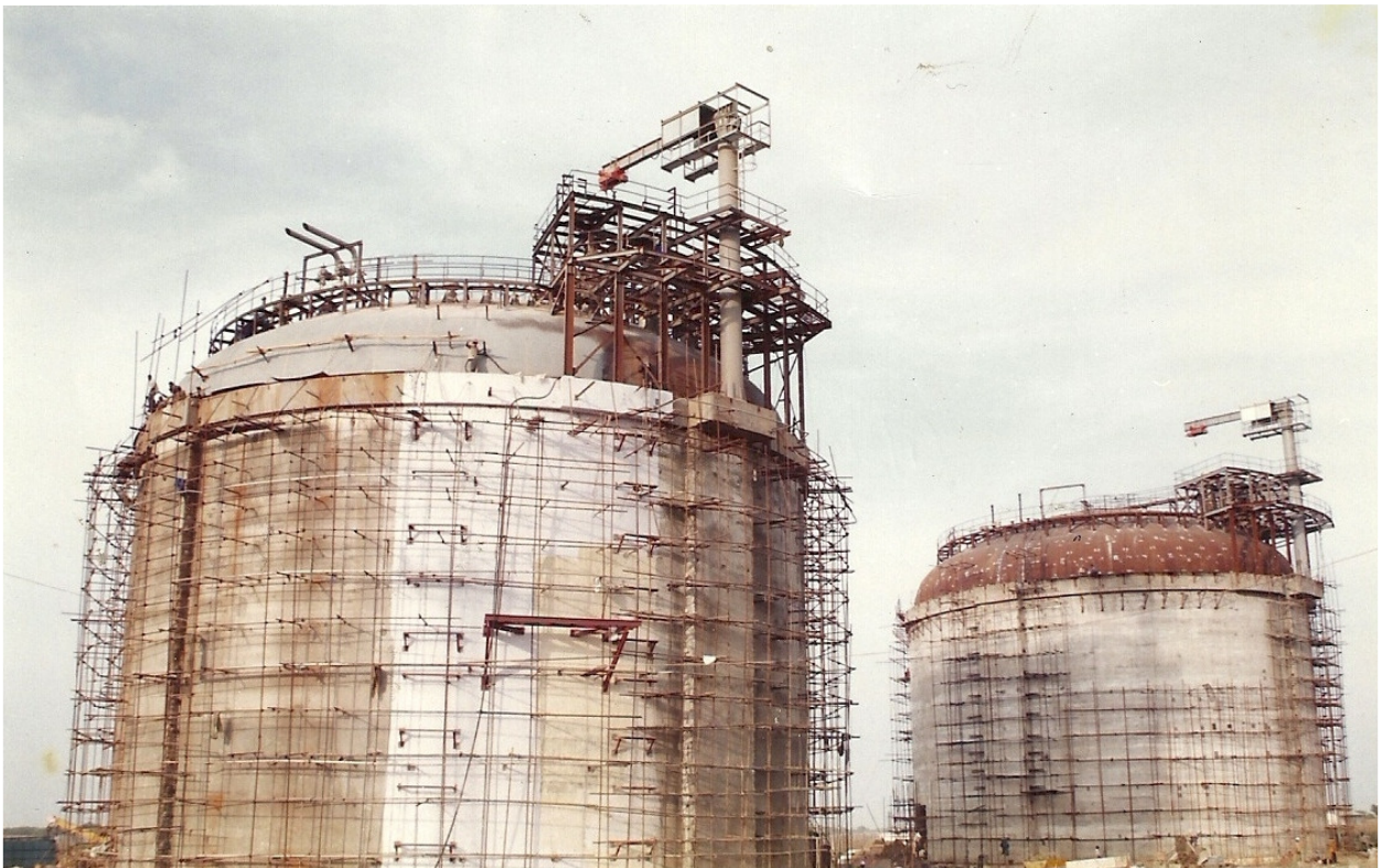
Completed view of tank with roof work in progress
